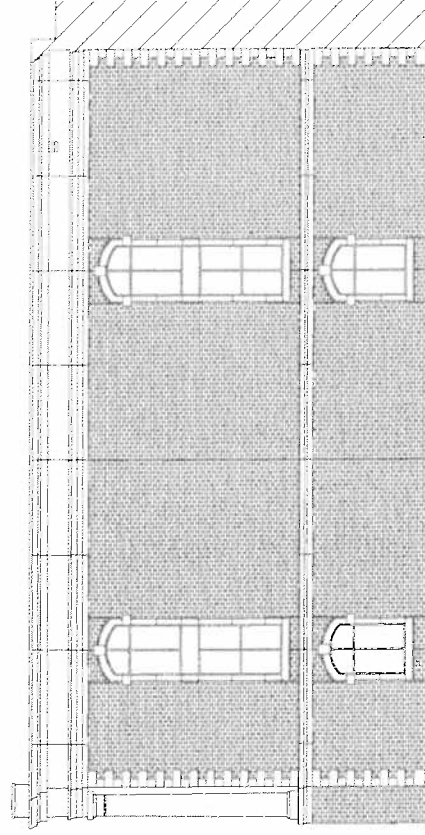
SOUTH ELEVATION
