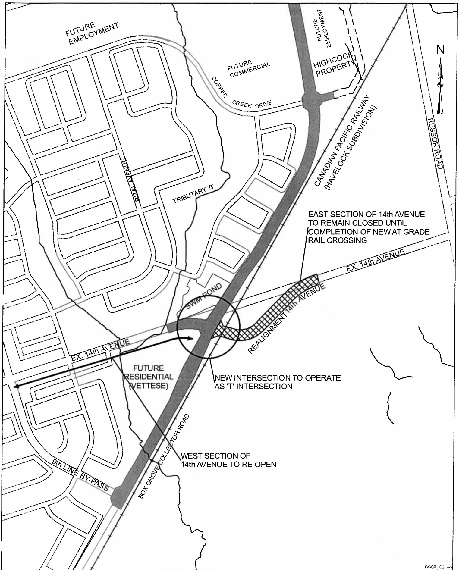
Attachment 'C' - Temporary Conditions to Open Box Grove Collector Road.
