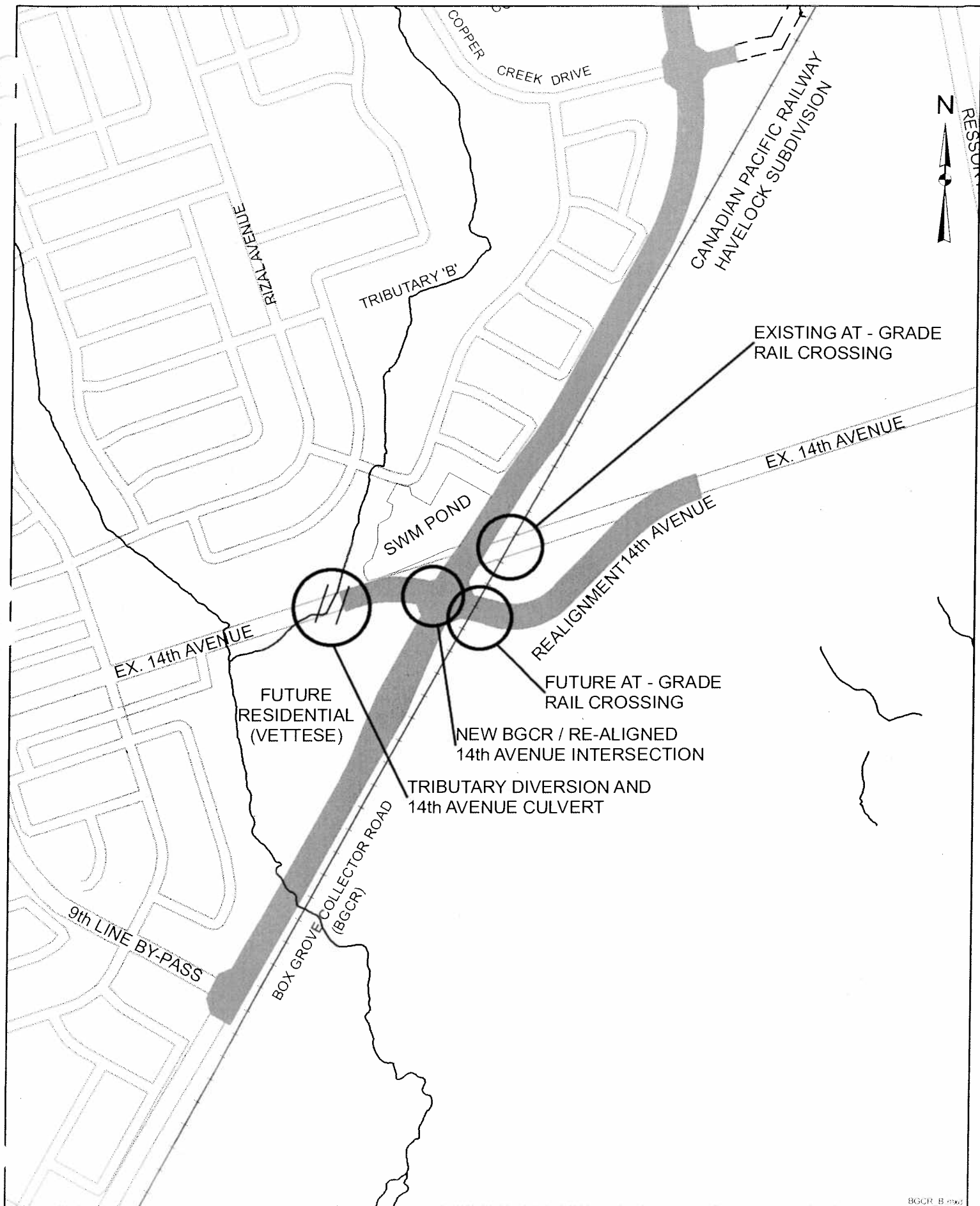
Attachment 'B' - BGCR Construction and 14th Avenue Realignment
